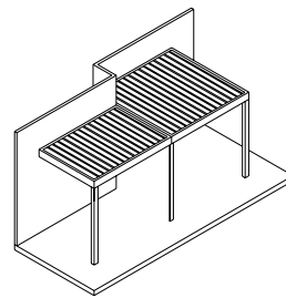
7 Wall-mounted blades perpendicular to wall
