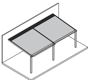
5 Wall-mounted Double module
